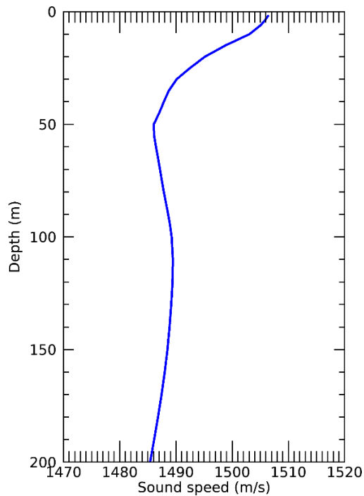
Figure K-3. Mean Sound speed profile up to 200 m for the summer months for New England Wind. The mean profile used in the modeling was obtained by taking the average of all profiles for June through August.
