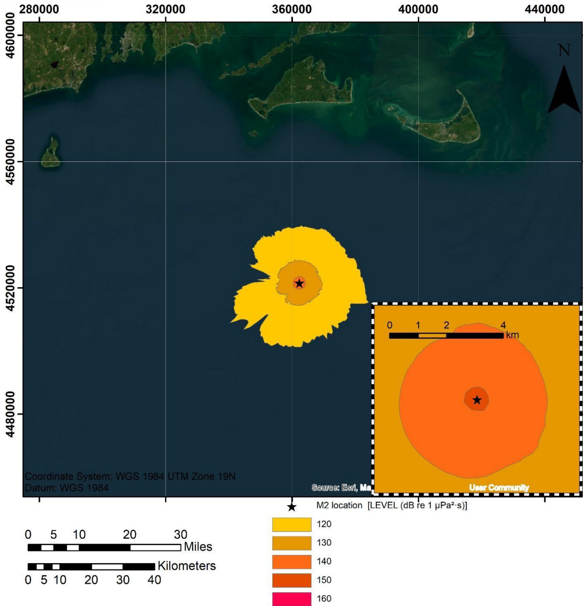
Figure K-10. Location M2 – Modeled unweighted sound exposure level for 24 hours of drilling.
