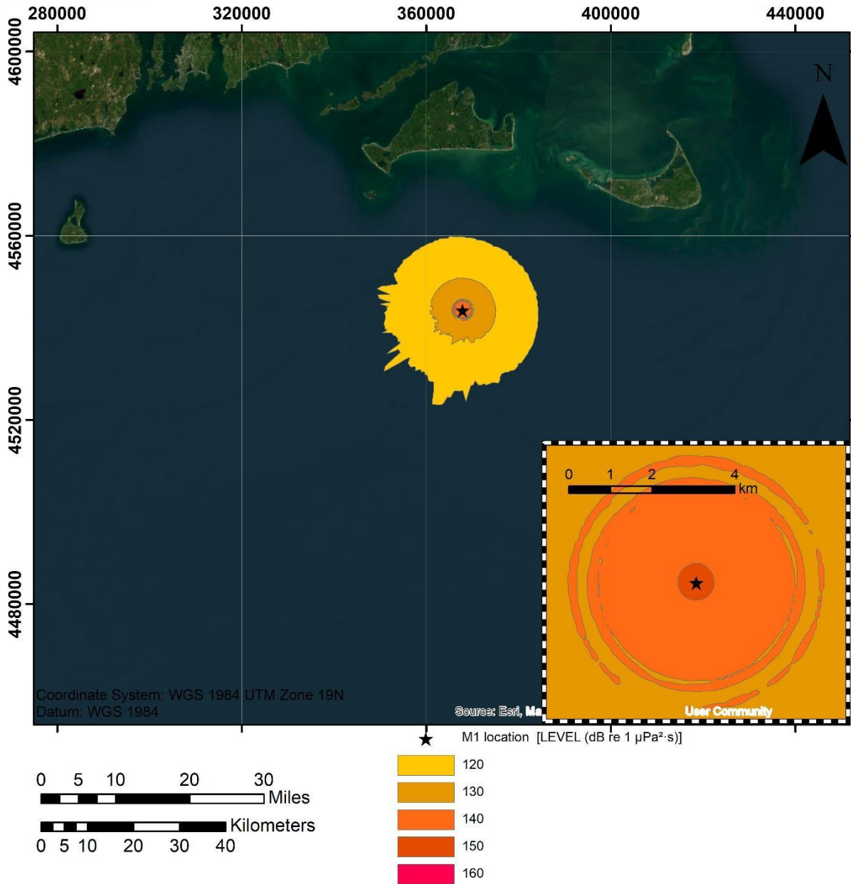
Figure K-9. Location M1 – Modeled unweighted sound exposure level for 24 hours of drilling.
