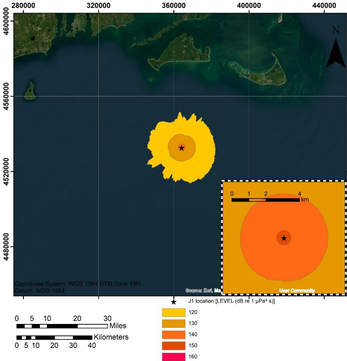
Figure K-8. Location J1 – Modeled unweighted sound exposure level for 24 hours of drilling.
