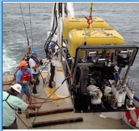
Recovering an ROV, by Melanie Damour, BOEM
