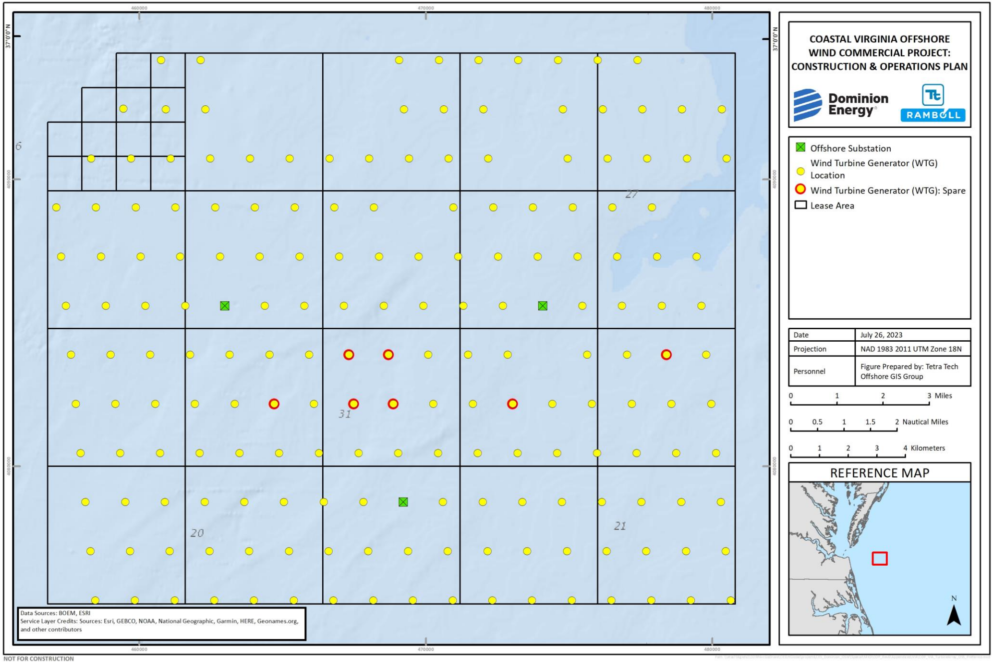
Figure I-1-1. WTG and Offshore Substation Preferred Layout
