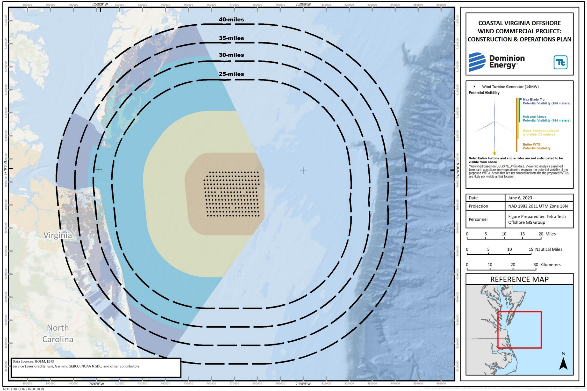
Figure I-1-9. Preferred Representative Wind Turbine Generator (14 MW) Indicative Layout Topographic Viewshed Analysis
