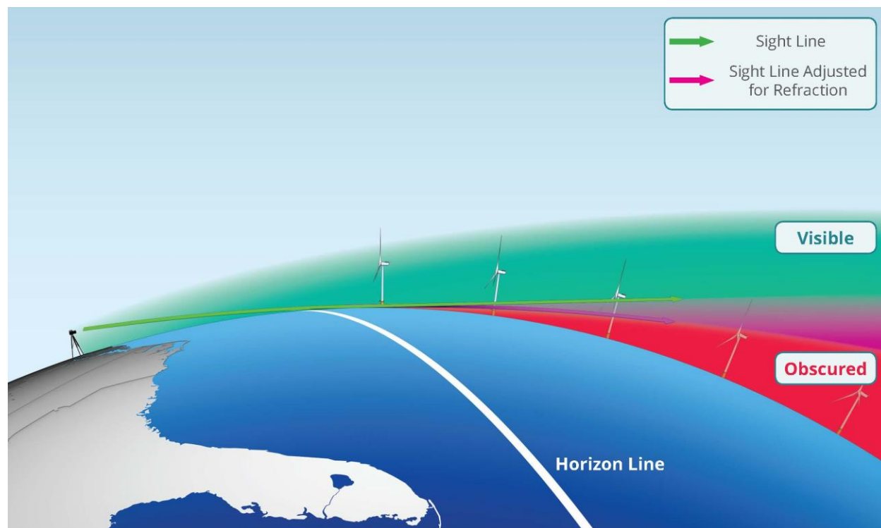
Figure I-1-20. The Effects of the Curvature of the Earth and Atmospheric Refraction on the Apparent Height of Objects
