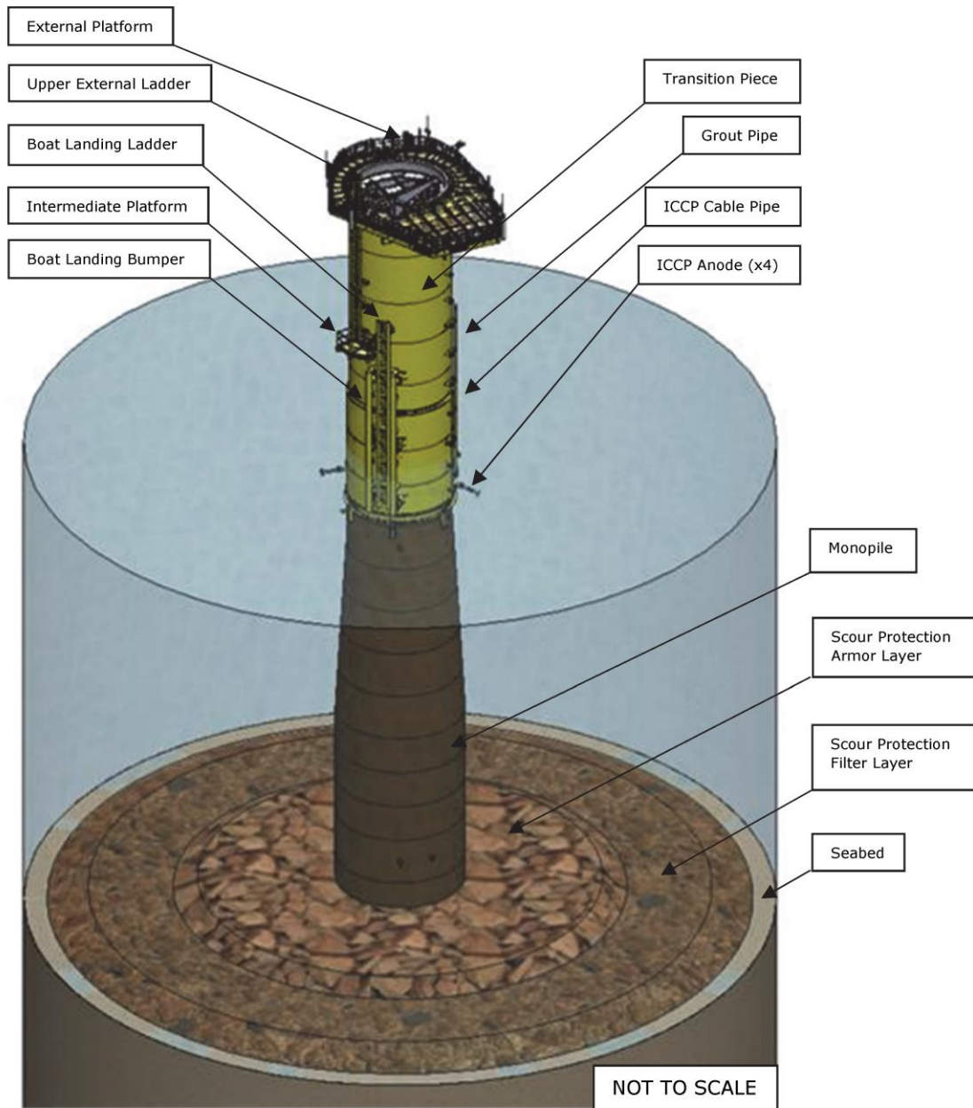
Figure I-1-4. Illustrative Example of the Wind Turbine Generator Monopile Foundation (Figure provided courtesy of Ramboll)
