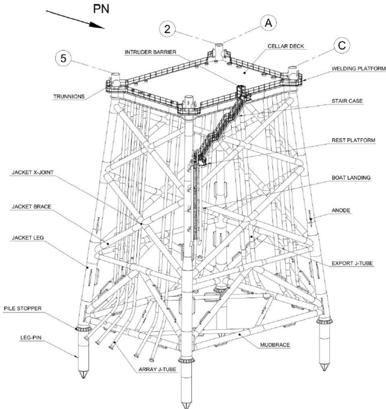
Figure I-1-5. Example Schematic of the Offshore Substation Jacket Foundation (Figure provided courtesy of Ramboll)
