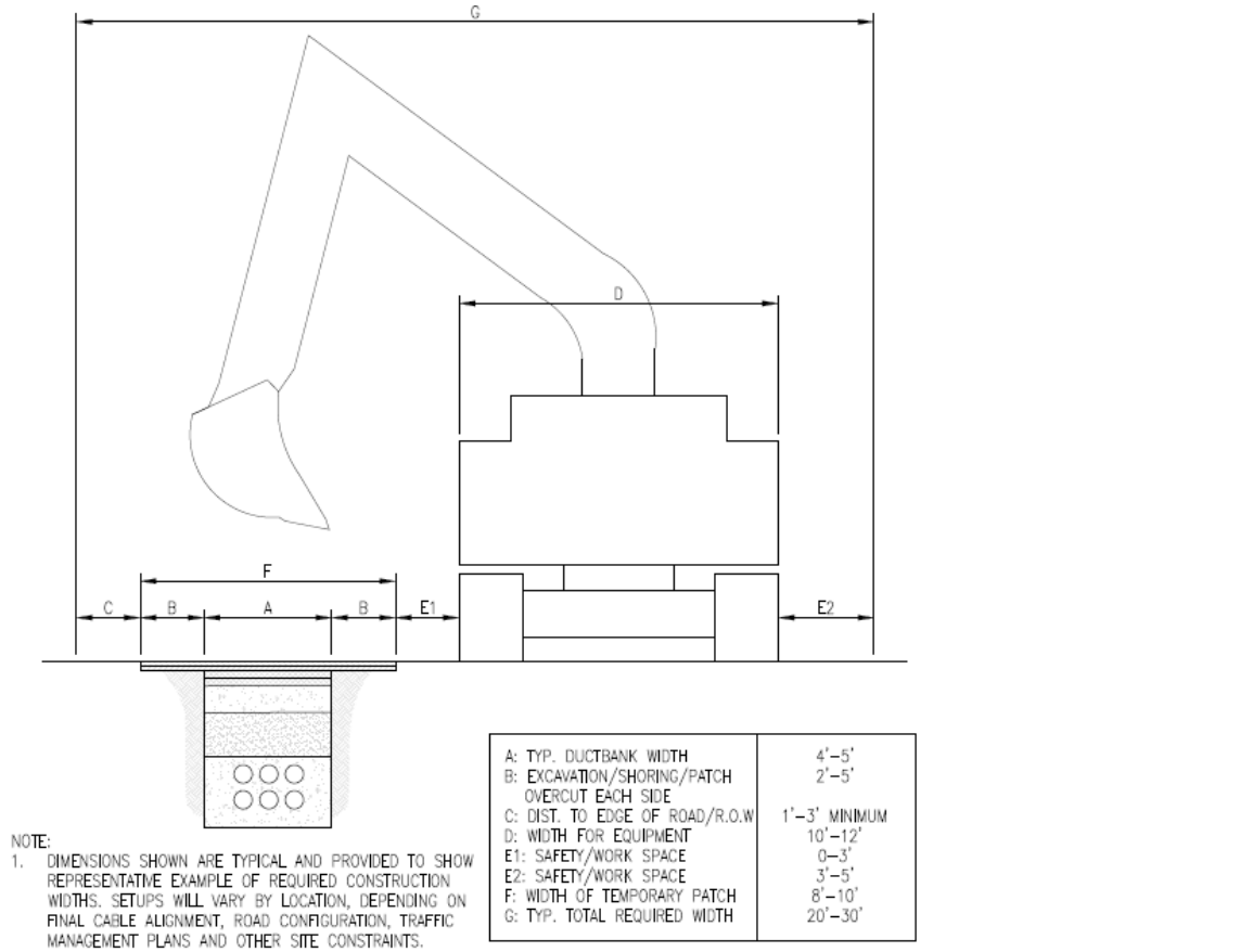
Figure 3.3.2-5 Typical Underground Onshore Transmission Circuit Installation within a Road Right-of-Way
