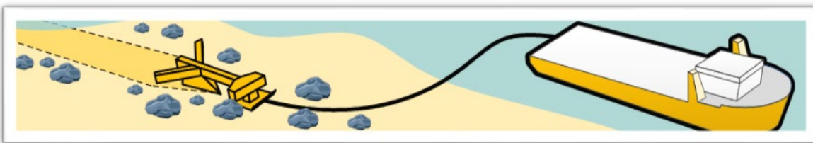
Figure 3.3.3-6 Typical Boulder Plow Configuration
