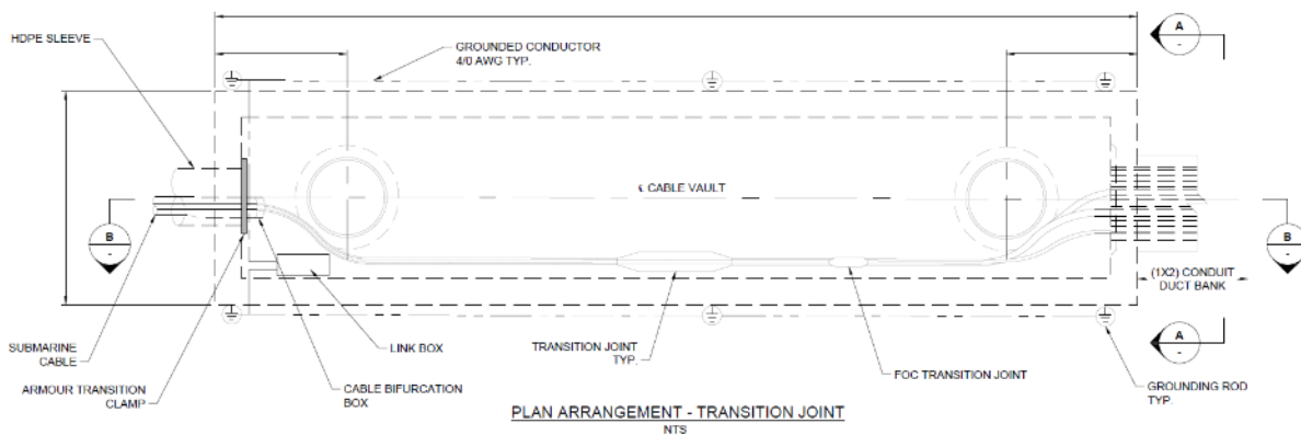
Figure 3.3.3-1 Example TJBs and Link Boxes
