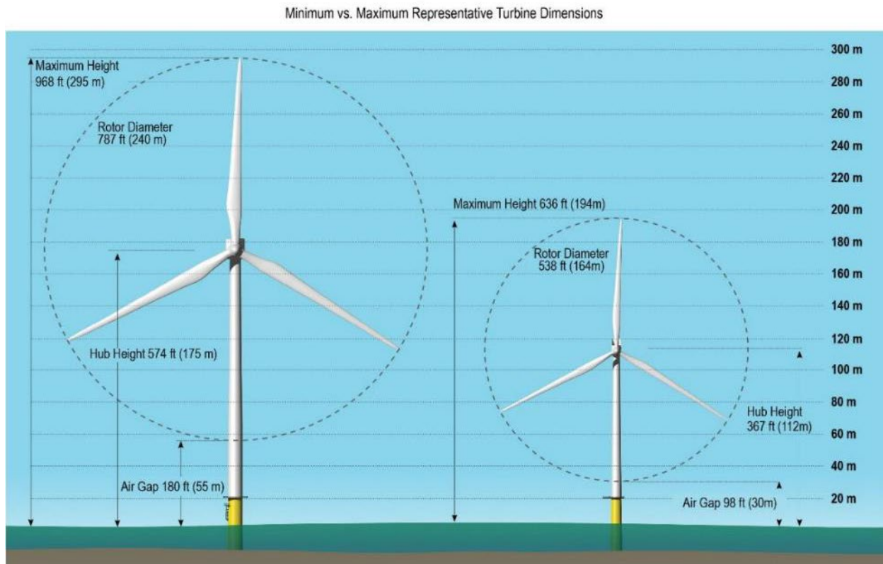
Figure 3.3.8-1 Conceptual Rendering of the Minimum and Maximum WTGs under Consideration
