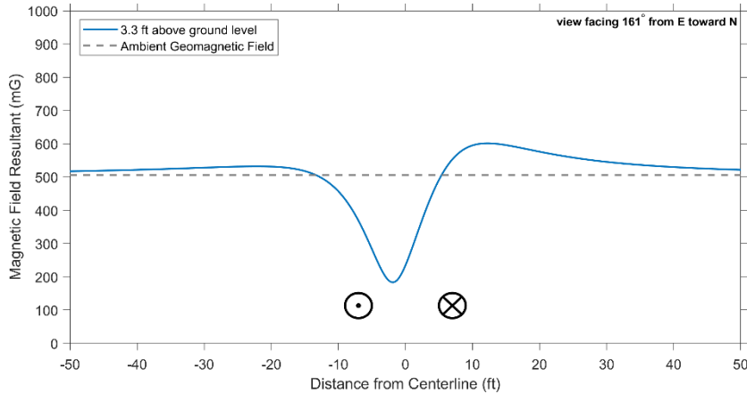
Figure C-10. Total DC magnetic field for SRWEC in which cables are installed horizontally separated at the TJB (TJB Option 2) and buried to a minimum depth of 7 ft (2.1 m) at WNC loading 3.3 ft (1 m) above the ground oriented 161 degrees north of east for two different current flow direction scenarios, indicated by the figure at the bottom center of each plot.
