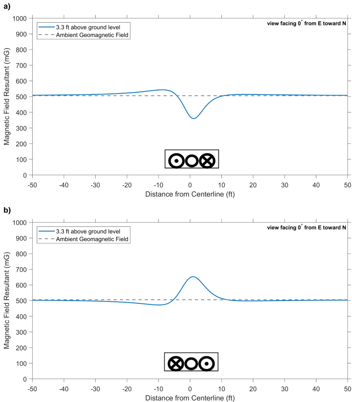
Figure C-1. Total calculated magnetic field at average loading for the Onshore Transmission Cable in the DC duct bank configuration for cables oriented along the east-west direction, evaluated at a height of 3.3 ft (1 m) above ground.
