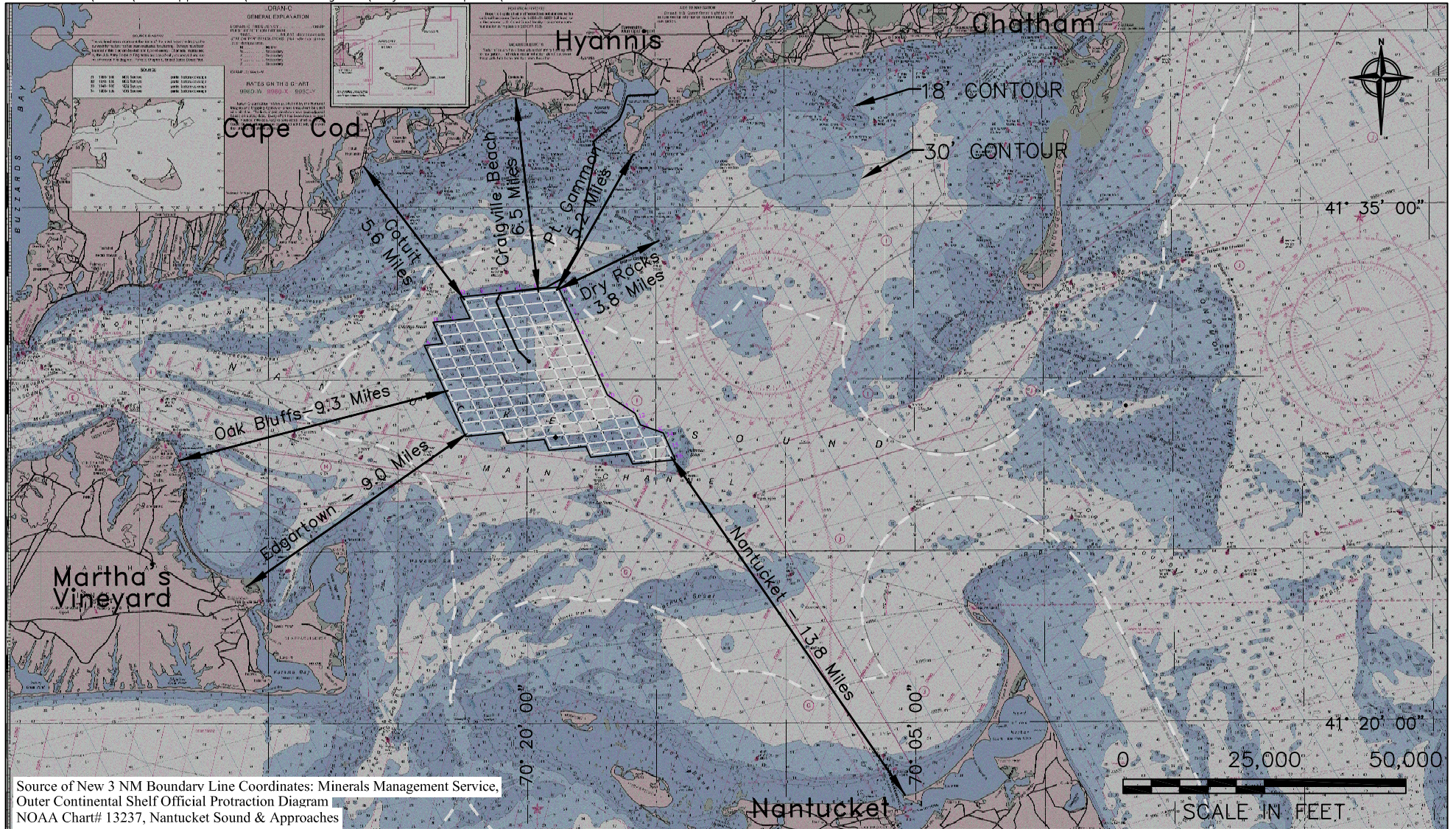
CAPE WIND ENERGY PROJECT Revised Turbine Array - New 3 Mile Boundary Figure 2.1.1-2
